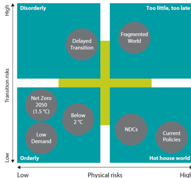
NGFS scenarios framework in Phase V
