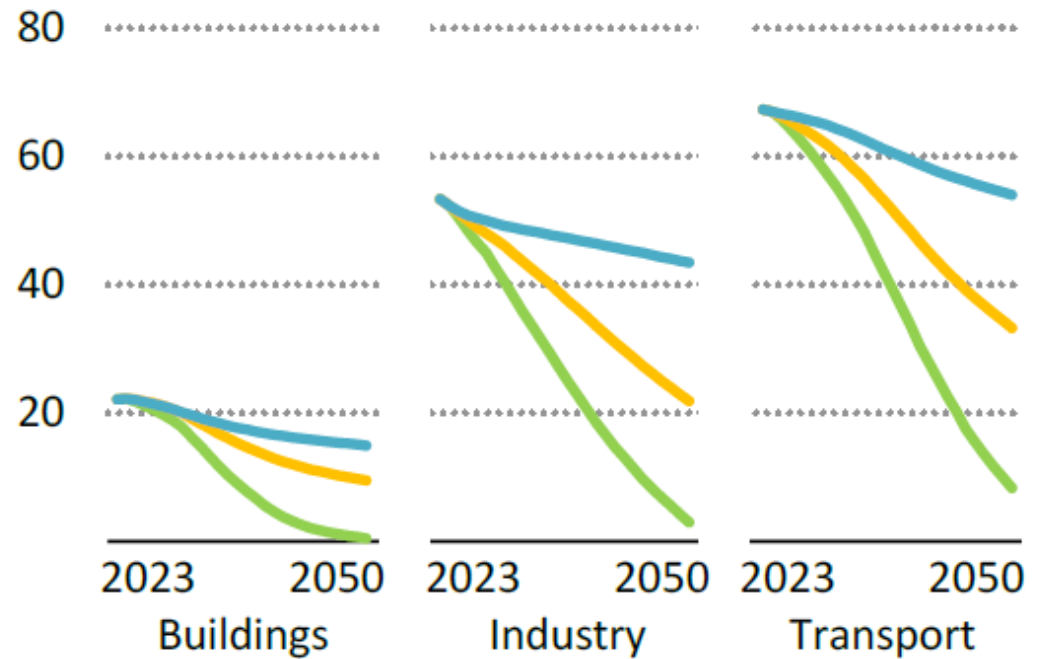
CO 2 emissions intensity (t CO 2 per TJ)
