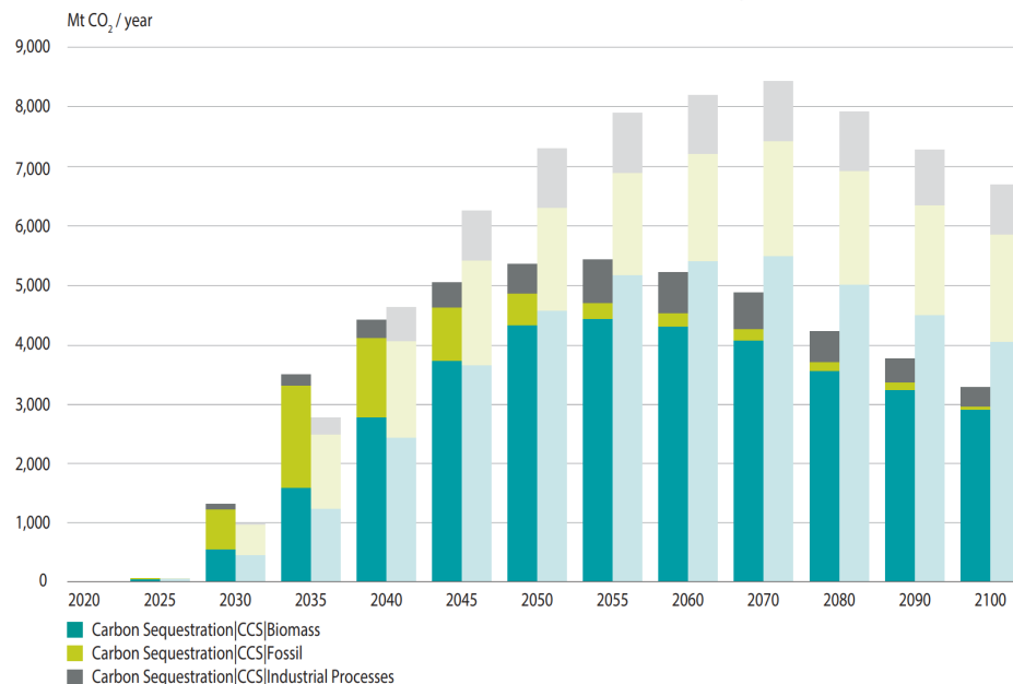
Carbon Sequestration Phase IV vs Phase III
