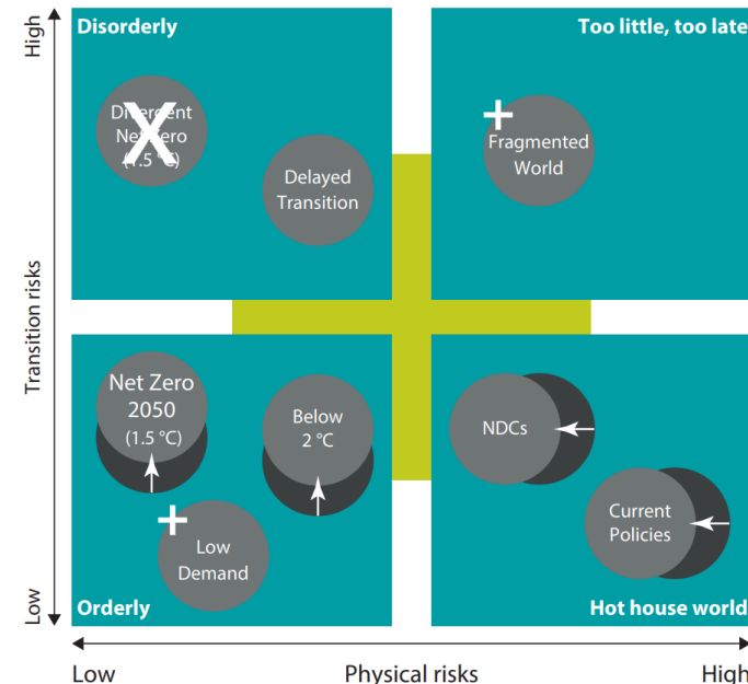
NGFS scenarios framework: from Phase III to Phase IV
