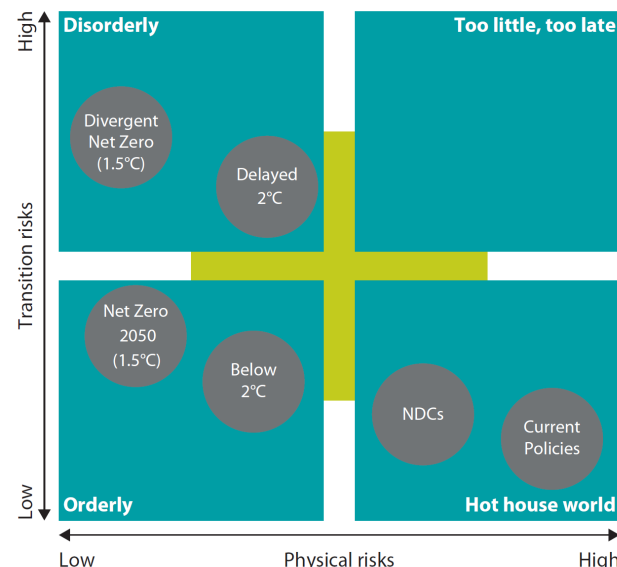
NGFS scenarios framework
