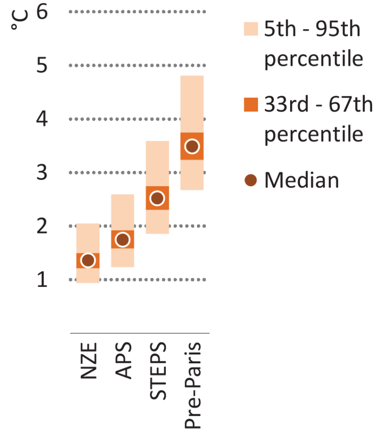
Temperature rise in 2100
