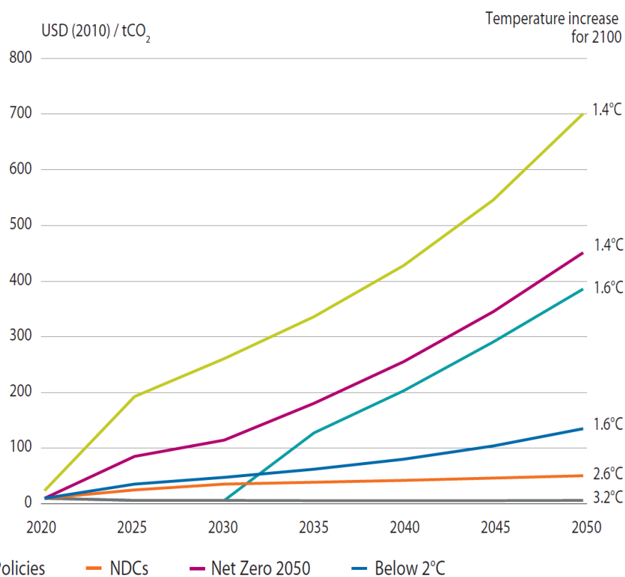
Carbon price development
