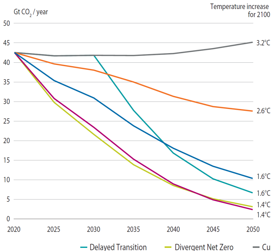
CO 2 emissions by scenario
