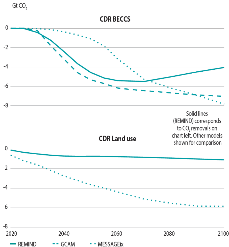
CO 2 removals across models
