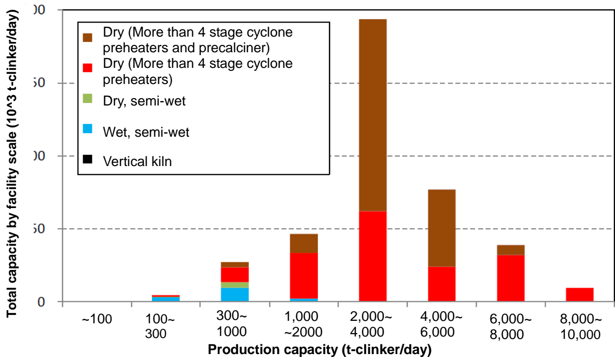
Fig.5 Total capacity by facility scale in India (2002)
