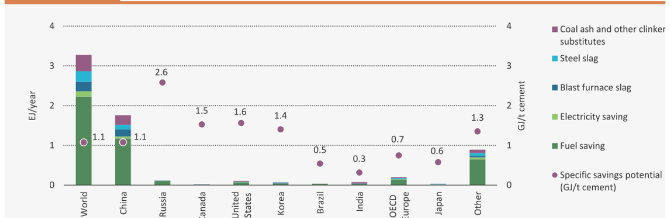
Fig.3 Regional energy saving potentials
